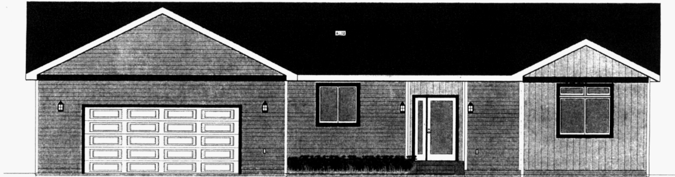
FRONT ELEVATION 1/4 in = 1 ft
