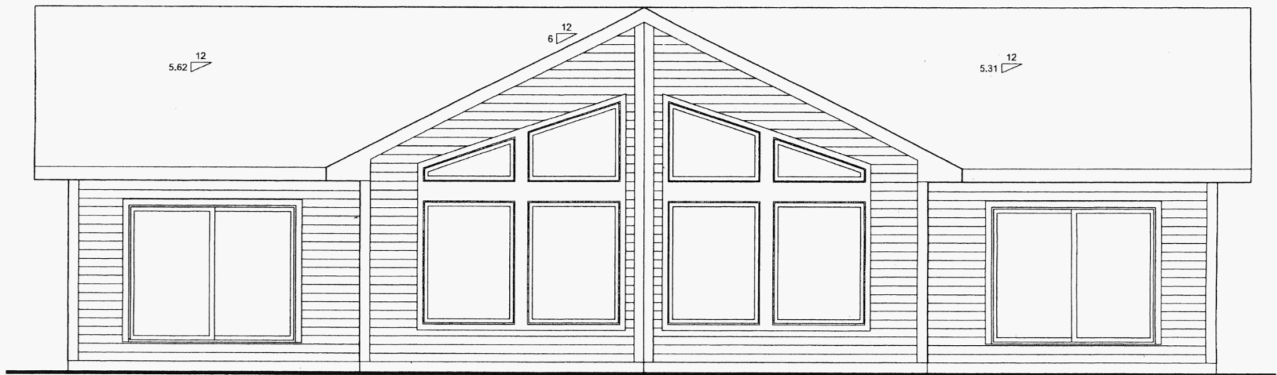
REAR ELEVATION 1/4"=1'-0"
