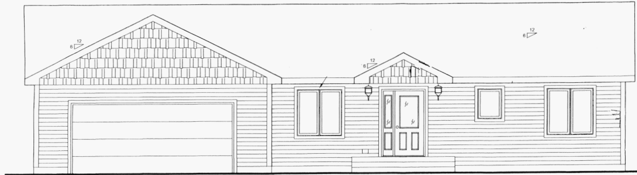
FRONT ELEVATION
