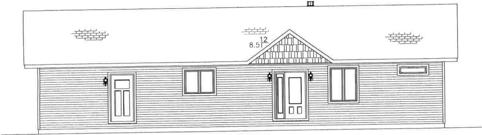
FRONT ELEVATION
