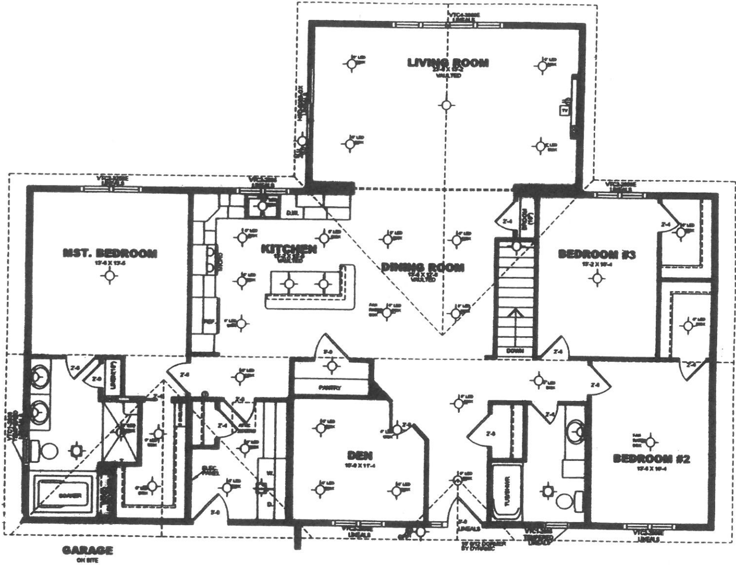
FLOOR PLAN 1/4" = 1'-0" (DIMENSIONS FRAMING TO FRAMING)
