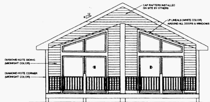
LEFT SIDE ELEVATION 1/4" = 1'-0"
