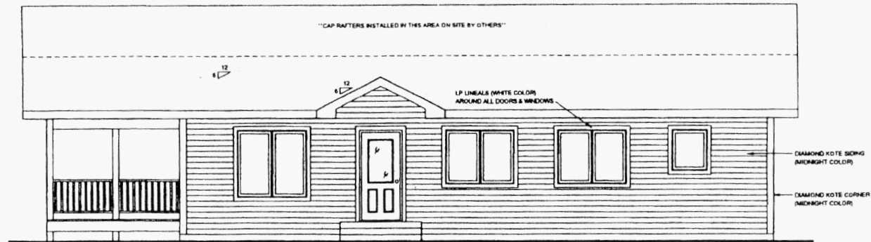
FRONT ELEVATION 1/4" = 1'-0"
