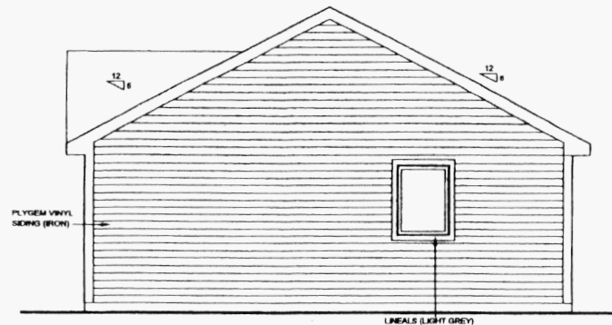
RIGHT ELEVATION 1/4"=1'-0"
