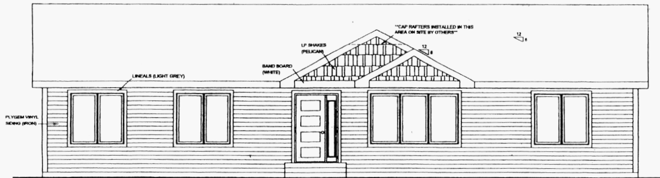
FRONT ELEVATION 1/4"=1'-0"
