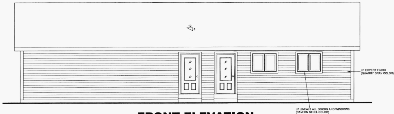
FRONT ELEVATION 1/4"=1'-0"
