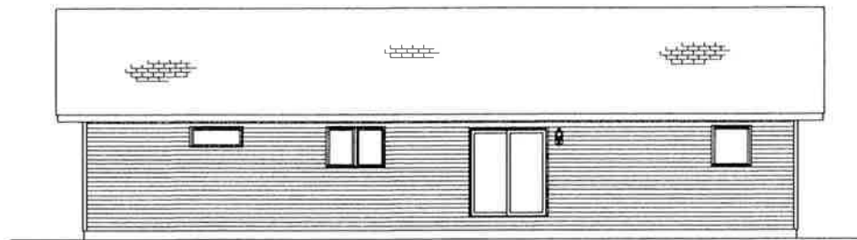
REAR ELEVATION
